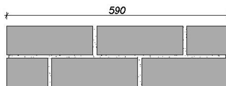
2 ½ brick pier
